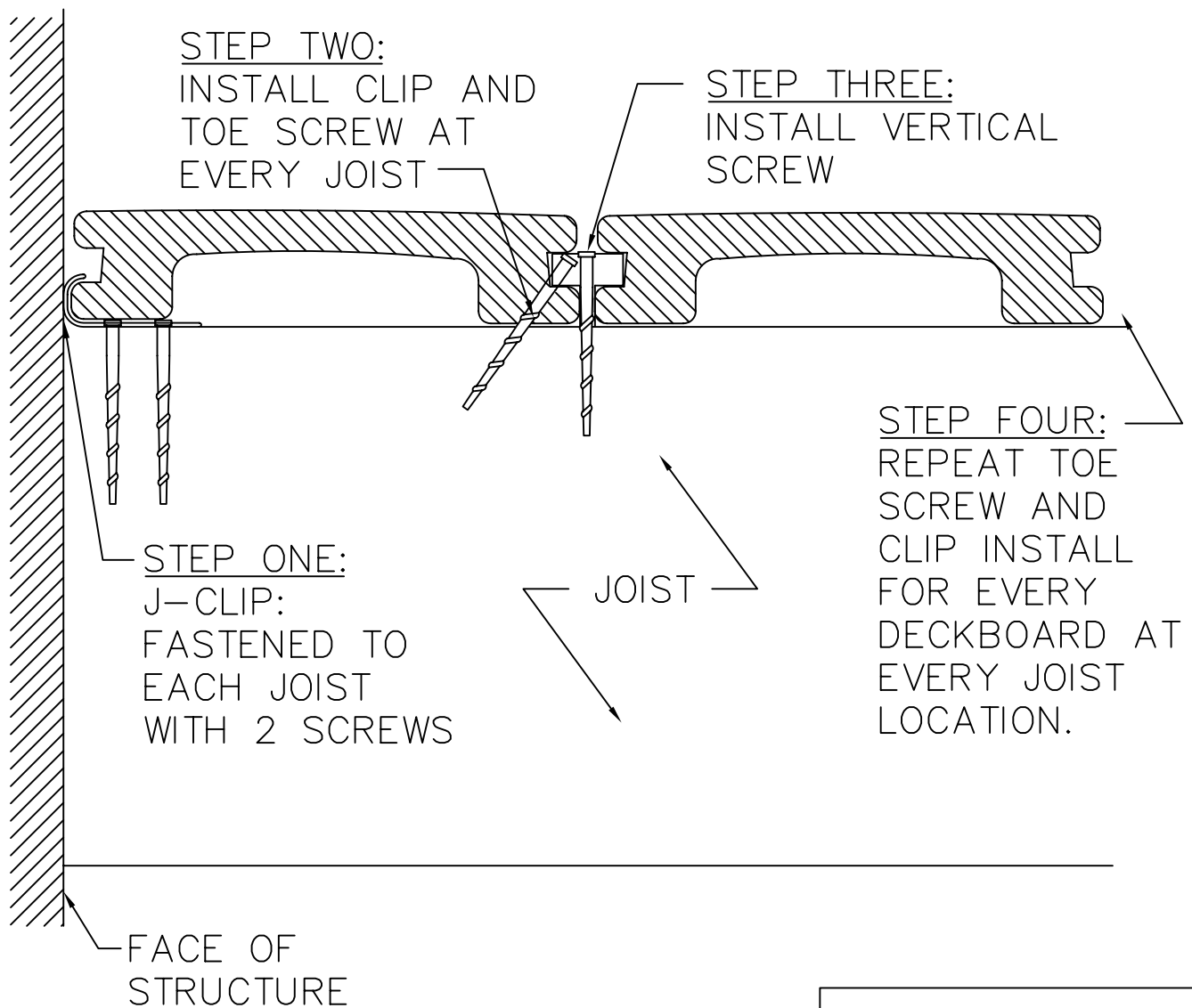
DECKING CLIP
