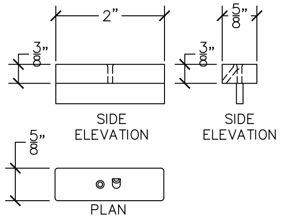
DECKING CLIP
